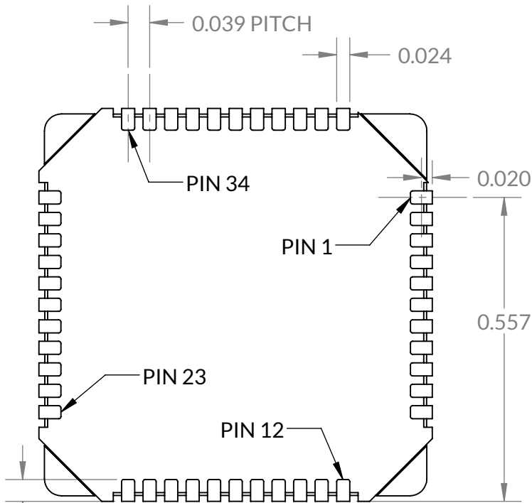
PAD DETAIL A
